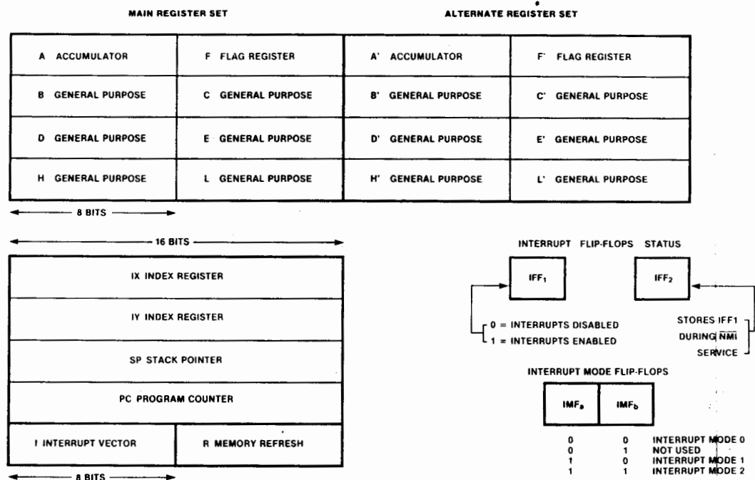
Figure 4. CPU Registers
